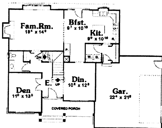
Main Floor
